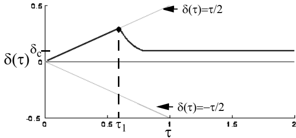
Figure 5: Representative \delta(\tau) curve. \delta(\tau) = \tau/2 for all \tau < \tau_1 .
